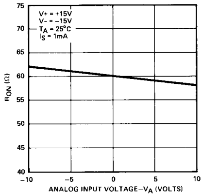
"ON" RESISTANCE vs ANALOG VOLTAGE ( V_A )
