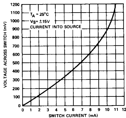
SWITCH CURRENT vs VOLTAGE
