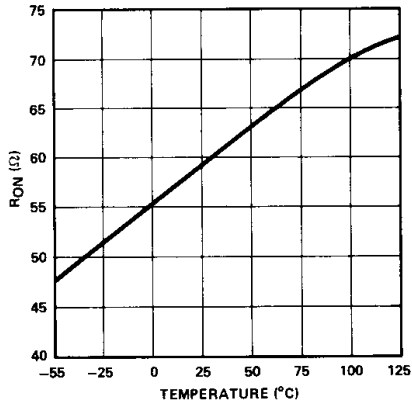
RON vs TEMPERATURE
