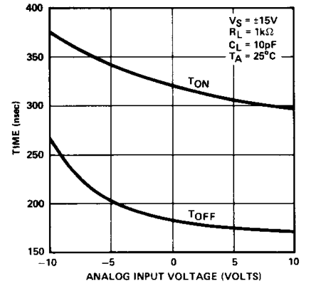
SWITCHING TIME vs ANALOG VOLTAGE
