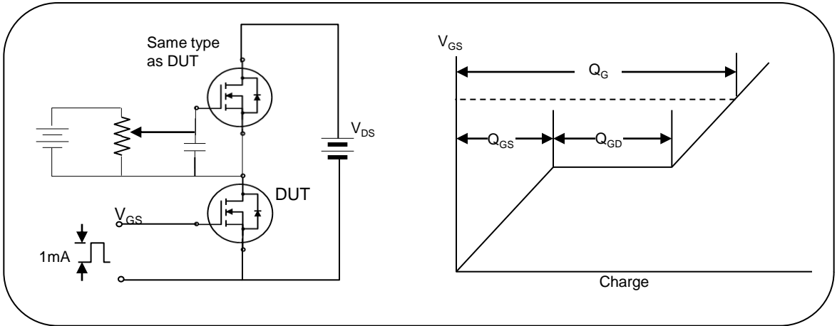
Fig. 1. Gate charge test circuit & waveform
