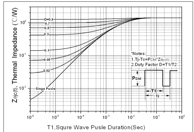
Fig. 8. Transient thermal response curve (TO-251)
