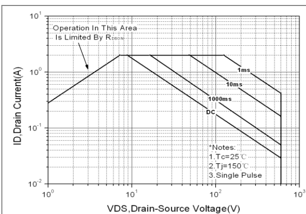
Fig. 11. Maximum safe operating area (TO-220F)
