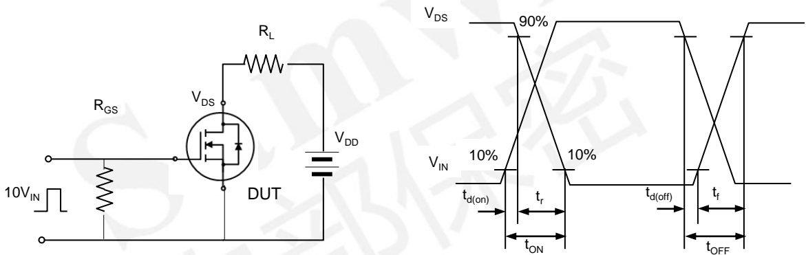
Fig. 12. Switching time test circuit & waveform
