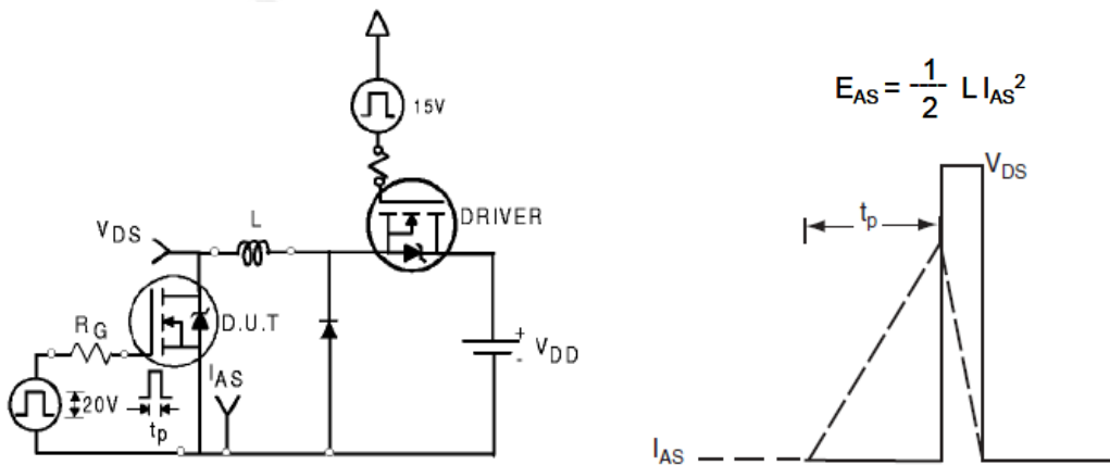
Fig. 13. Unclamped Inductive switching test circuit & waveform
