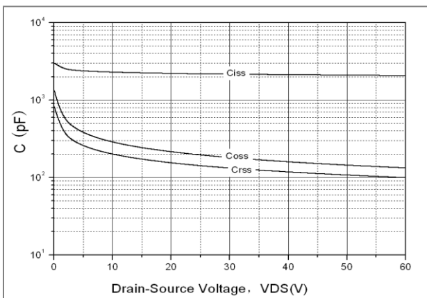
Fig. 11. Capacitance Characteristics
