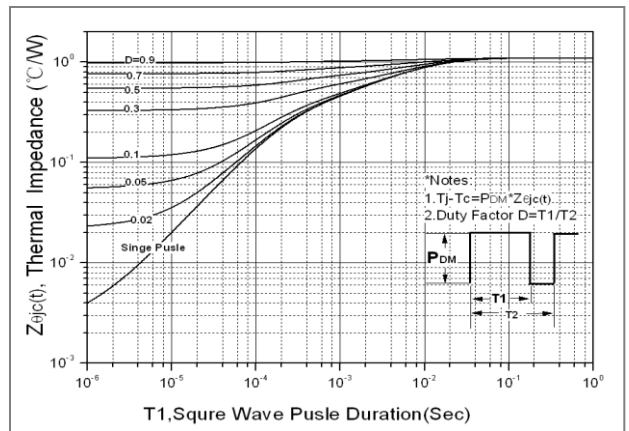
Fig. 10. Transient thermal response curve (TO-220)
