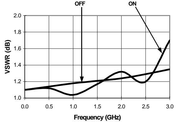
Typical VSWR
