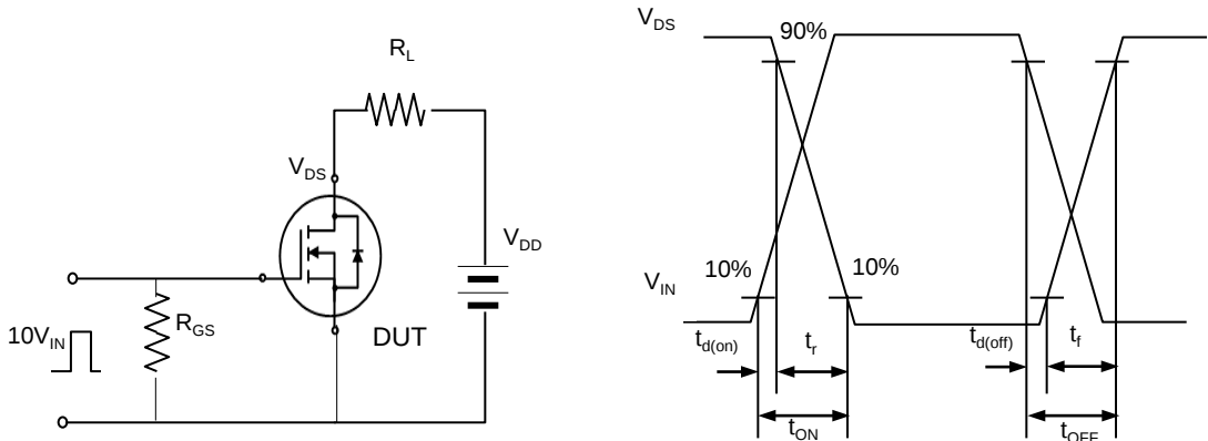
Fig. 13. Switching time test circuit & waveform
