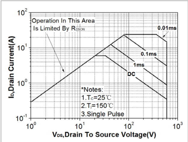
Fig. 8. Maximum safe operating area (TO-252&TO-251N)
