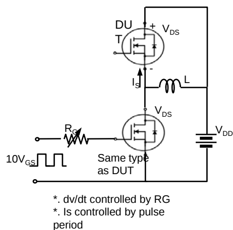
Fig. 17. Peak diode recovery dv/dt test circuit & waveform
