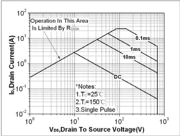
Fig. 9. Maximum safe operating area (TO-251N)
