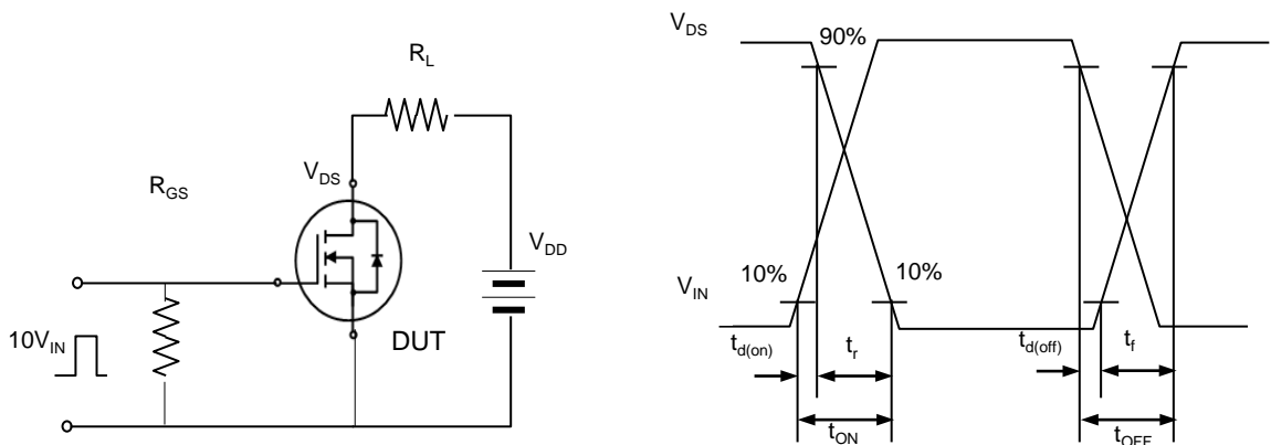
Fig. 14. Switching time test circuit & waveform
