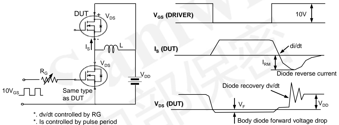
Fig. 16. Peak diode recovery dv/dt test circuit & waveform
