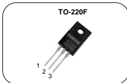
1. Gate 2. Drain 3. Source
