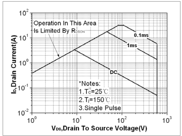
Fig. 8. Maximum safe operating area(TO-220F)
