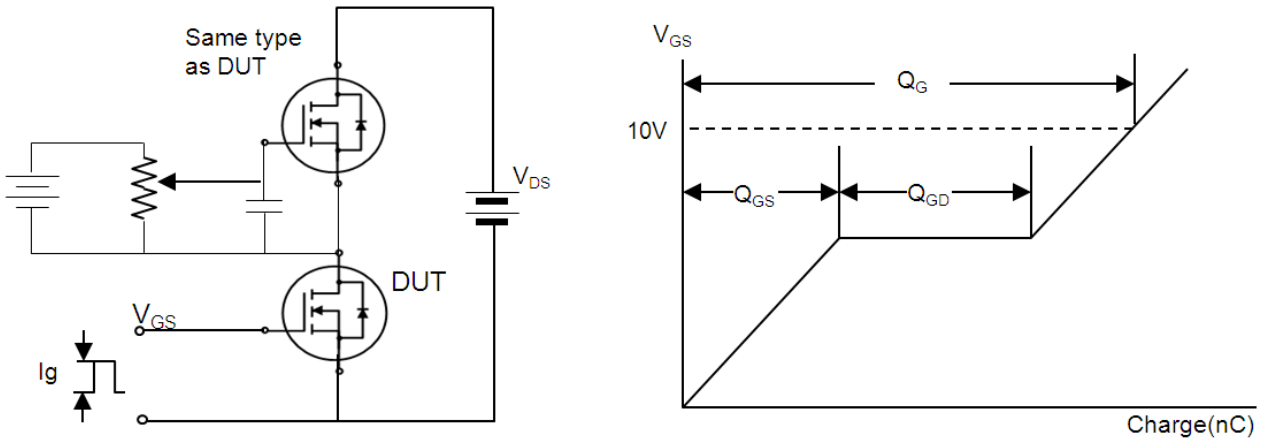
Fig. 10. Gate charge test circuit & waveform
