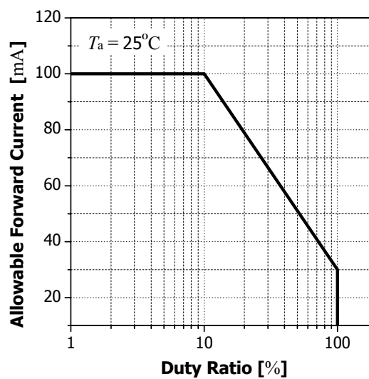
Allowable Forward Current vs. Duty Ratio
