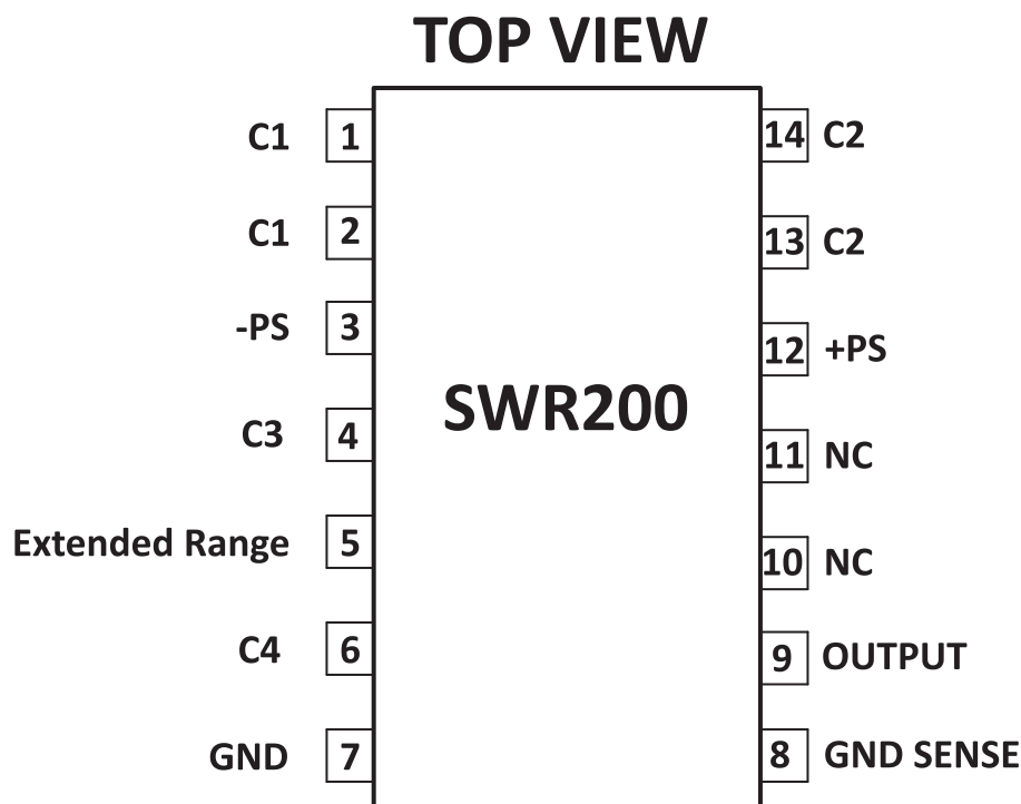
Figure 13: Pin Configuration
