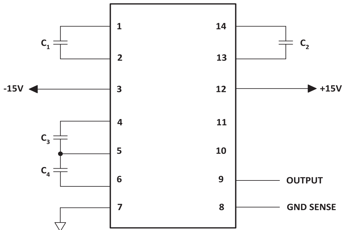
Figure 1: Typical Connection
