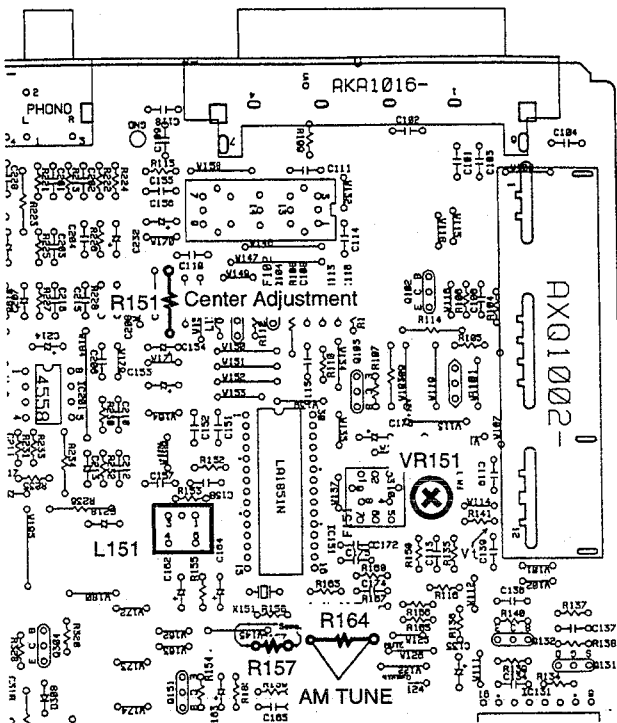
Fig. 1-2 Adjustment Points
