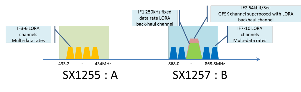
Figure 11: Radio Spectrum
