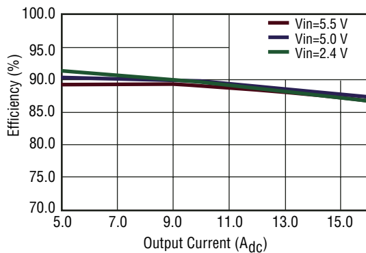
Fig. 3 Efficiency vs. Output Current ( V_{out} = 1.5 V_{dc} )
