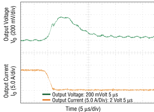
Fig. 11 Transient Response - 16 A - 8 A Step ( V_o = 3.3\text{ V}_{dc} )
