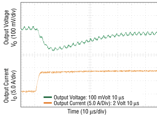
Fig. 12 Transient Response - 8 A - 16 A Step ( V_o = 3.3\text{ V}_{dc} , C_{ext} = 3 \times 100\text{ }\mu\text{F} Polymer Capacitors)
