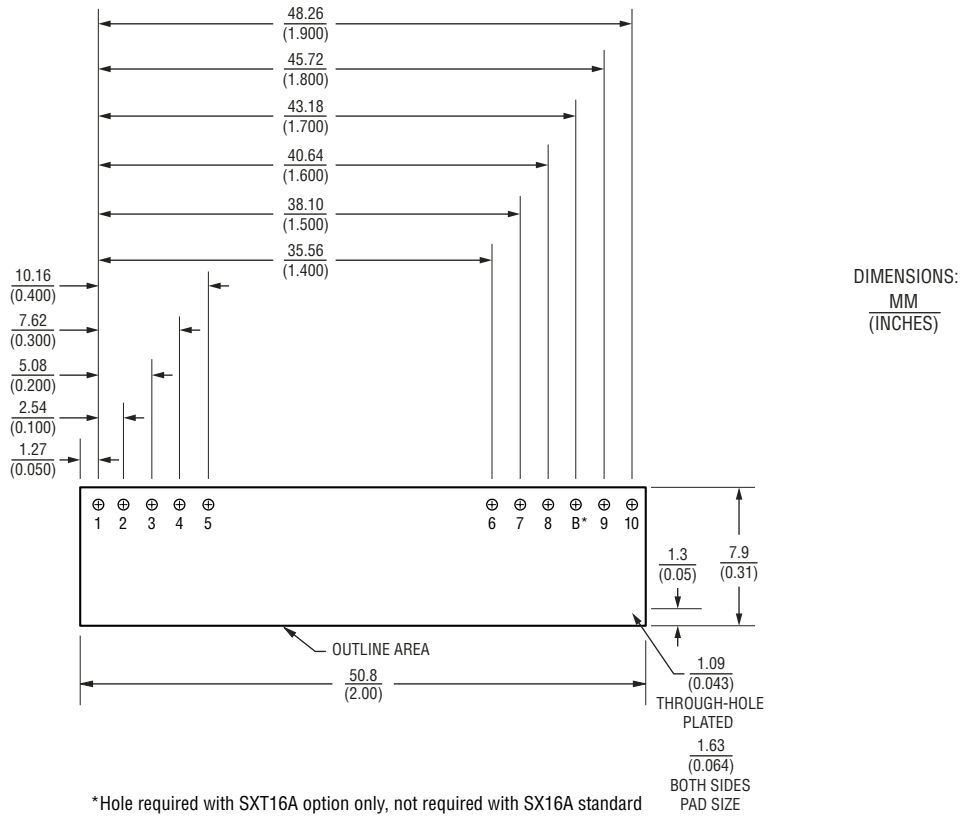
Fig. 33 Recommended Hole Pattern
