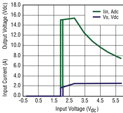
Fig. 7 Input Voltage vs. I_o and V_o ( V_o = 2.5\text{ V} , I_o = 16.0\text{ A} )
