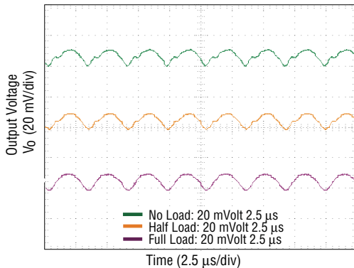
Fig. 8 Typical Output Ripple and Noise ( V_{in} = 5.0\text{ V} , V_o = 0.75\text{ V} , I_o = 16.0\text{ A} )
