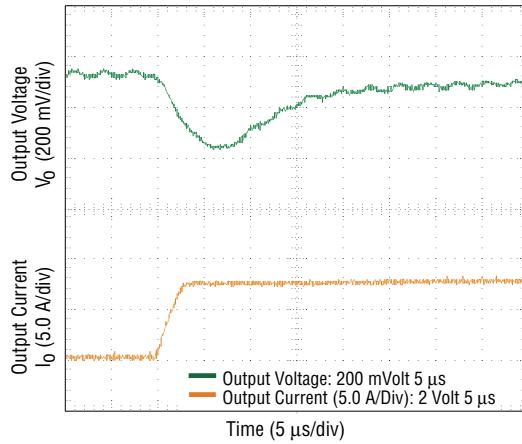
Fig. 10 Transient Response - 8 A - 16 A Step ( V_o = 3.3\text{ V}_{dc} )
