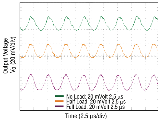
Fig. 9 Typical Output Ripple and Noise ( V_{in} = 5.0\text{ V} , V_o = 3.3\text{ V} , I_o = 16.0\text{ A} )
