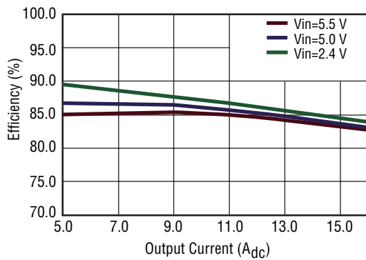
Fig. 2 Efficiency vs. Output Current ( V_{out} = 1.2 V_{dc} )
