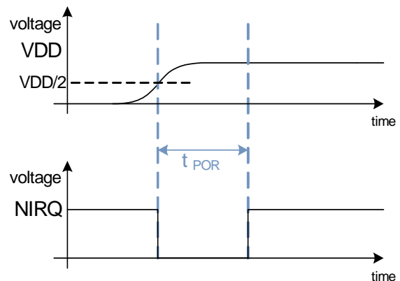
Figure 14. Power-up, NIRQ
