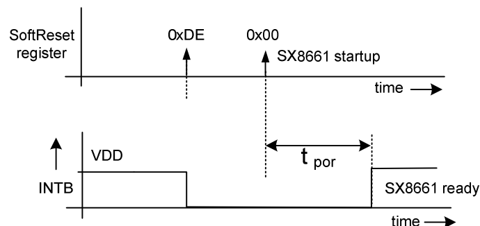
Figure 27 Software Reset
