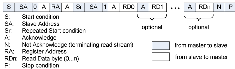
Figure 57 I2C read
