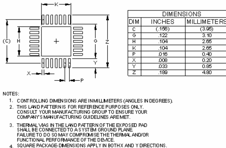
Figure 73 Land pattern
