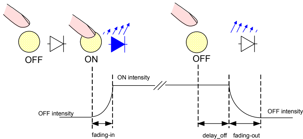
Figure 37 Single Fading Mode
