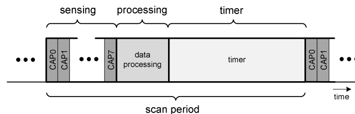
Figure 8 Scan Period
