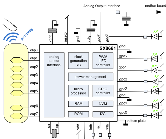
Figure 6 Quickstart Application
