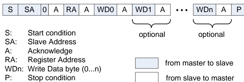
Figure 54 I2C write
