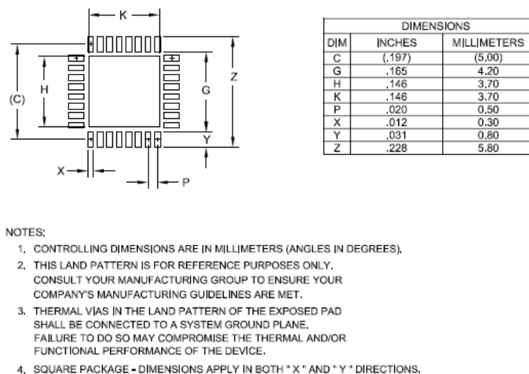
Figure 55 Land Pattern
