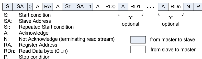
Figure 47 I2C read
