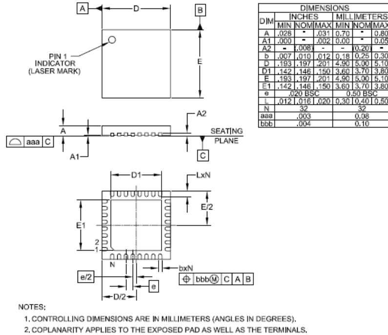
Figure 54 Package Outline Drawing
