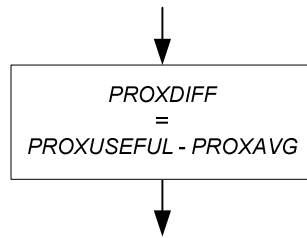
Figure 40 – ProxDiff Update
