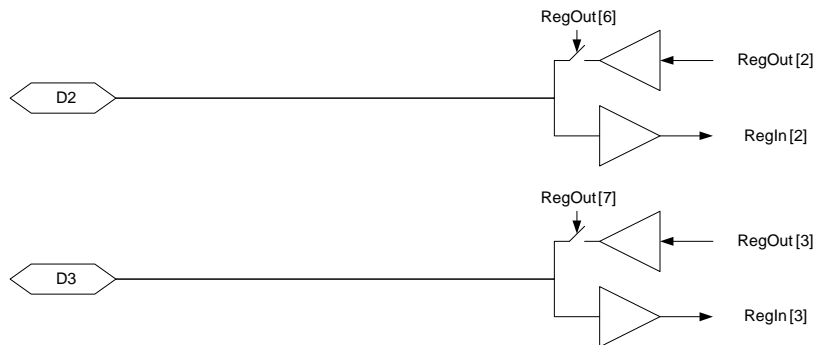
Figure 5. Digital IO bloc diagram
