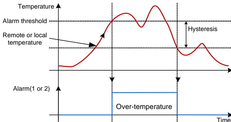
Figure 8. Alarm Output
