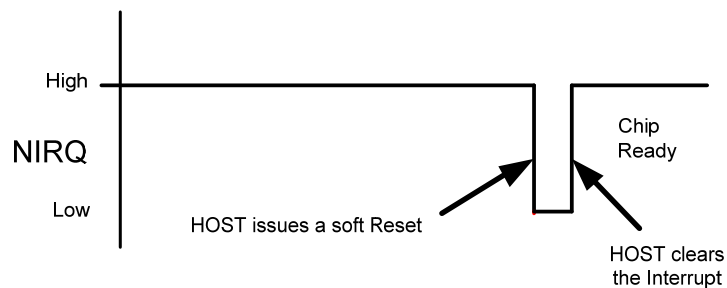
Figure 26: Software Reset
