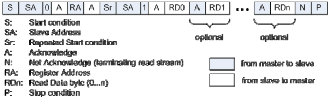
Figure 23: I2C Read
