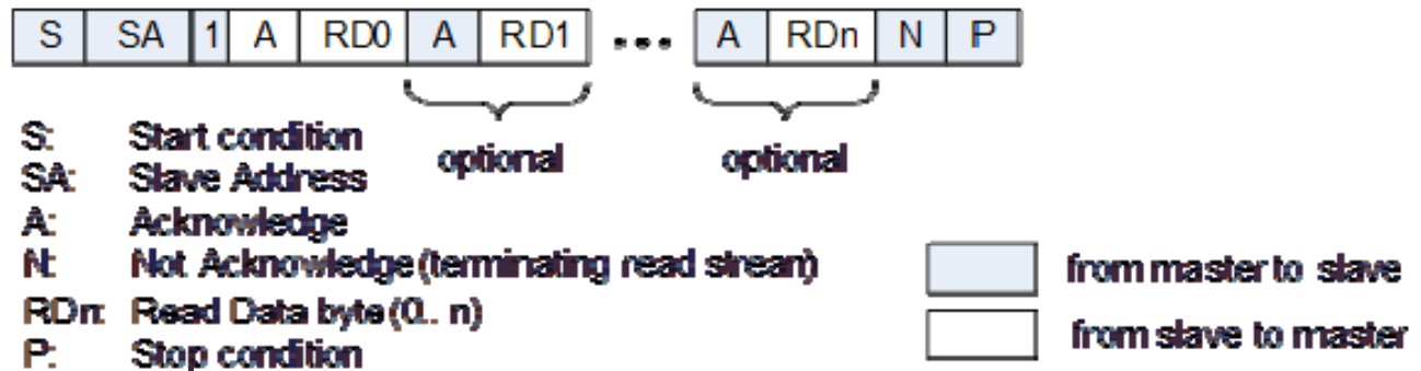
Figure 24: I2C Immediate Read
