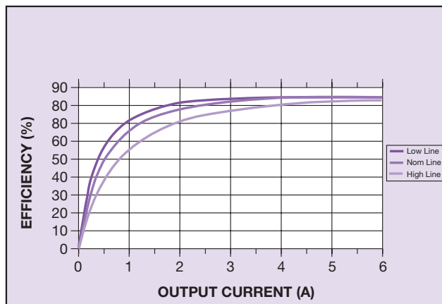
Figure 17: Efficiency vs. Load
