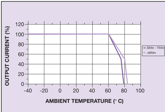
SXE15-48S3V3 Model
