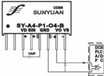
I/V Converter 2
