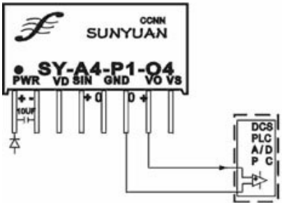
I/V Converter 1
