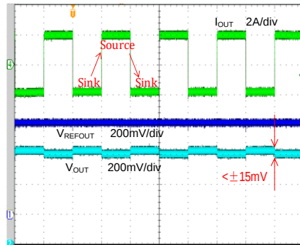
Load Transient
