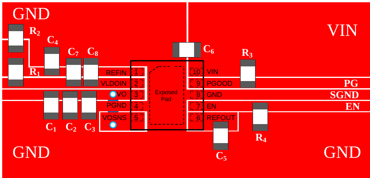
Figure 3. SY20735DBC PCB Layout Suggestion
