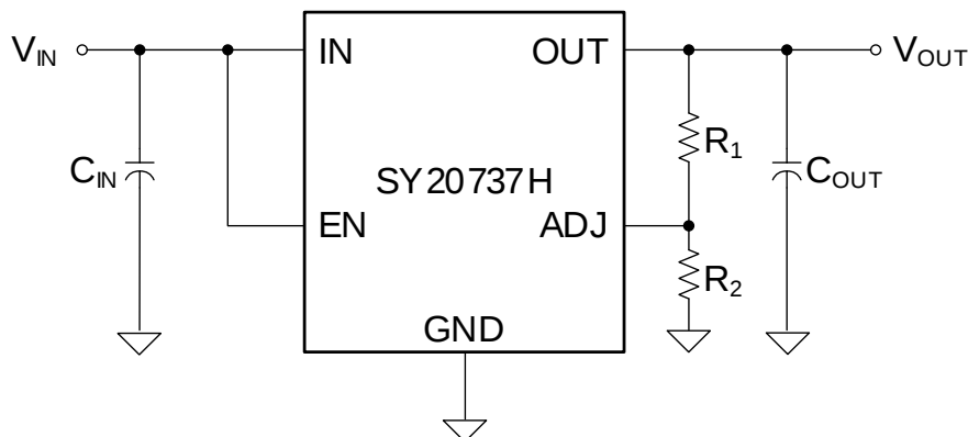
Figure 1. Schematic Diagram
