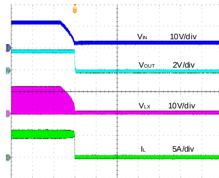
Shutdown from V_{IN} ( V_{IN}=12V, V_{OUT}=1.8V, I_{OUT}=6A , CCM)
