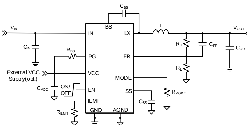
Figure1. Application Circuit
