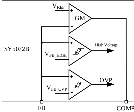
Figure 7. Output protection circuit
