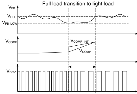
Figure 10. Load transition (Light load to full load)
