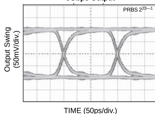
10.7Gbps Output
