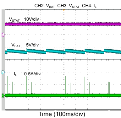
Steady waveform when no battery (NTC=50% V IN , No battery)
