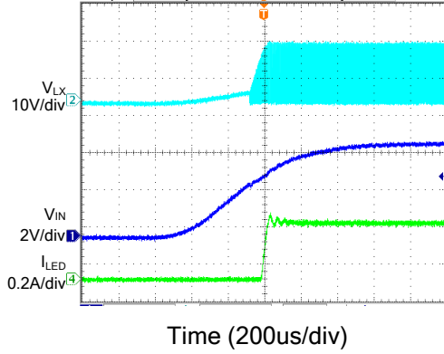
Starup from V_{IN}
