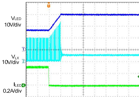
Time (20us/div)
