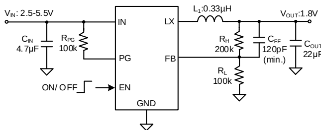
Figure1. Schematic Diagram
