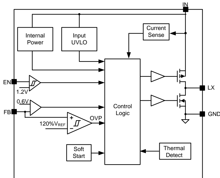
Figure3. Block Diagram
