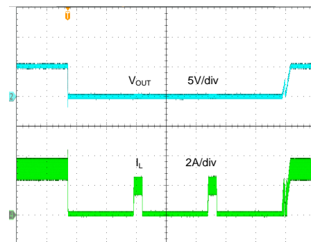
Short Circuit Protection ( V_{IN}=24V , V_{OUT}=5V , I_{OUT}=3A - Short)
