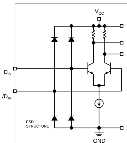
Figure 2. Input Structure
