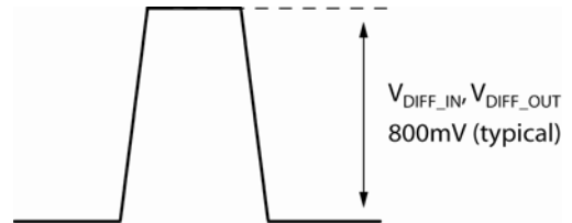
Figure 5b. Differential Voltage Swing
