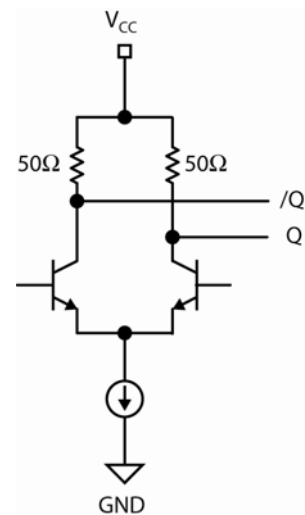
Figure 7. CML Output Stage
