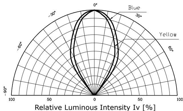
Fig. 5 Radiation Diagram
