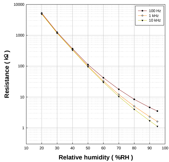
Fig. 4. Frequency characteristics
