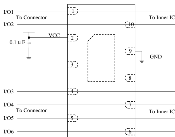
Figure 1 SYT07S05 pin connection in PCB providing data lines and power rail line protection.
