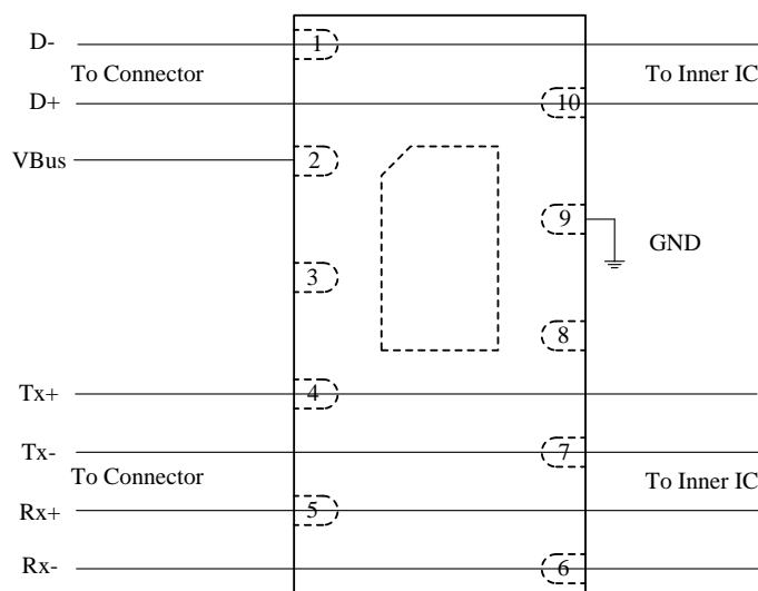
Figure 3 SYT07S05 pin connection for USB3.0 protection.
