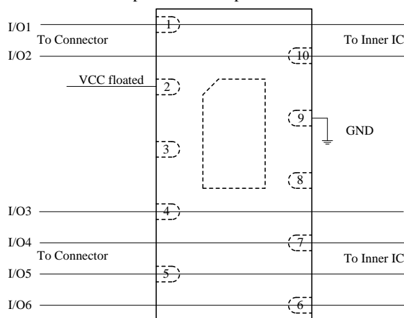
Figure 2 SYT07S05 pin connection in PCB providing data line protection. VCC pin is left as floating when no VCC rail is presented in PCB.
