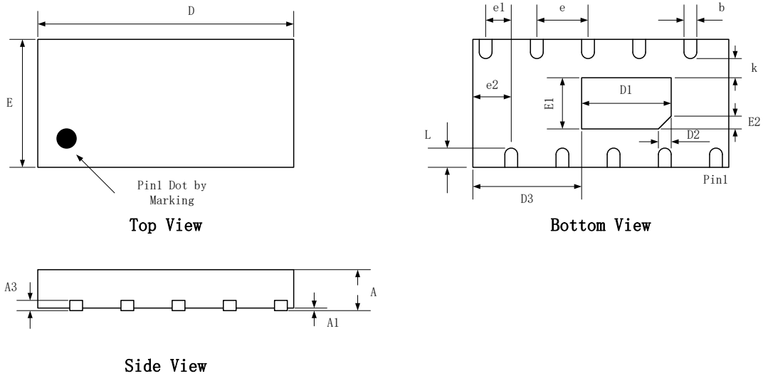
Package Dimensions (Controlling dimensions are in millimeters)
