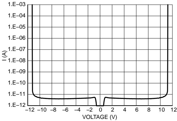
Figure 1. IV Characteristics
