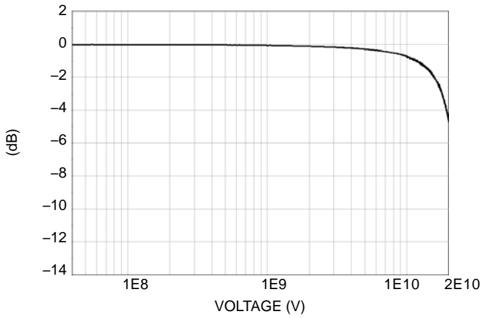
Figure 3. RF Insertion Loss
