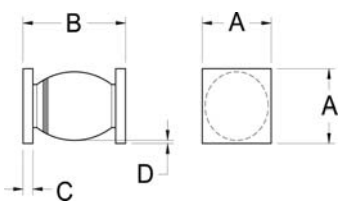
AXIAL ( K & ) All dimensions are prior to soldering
