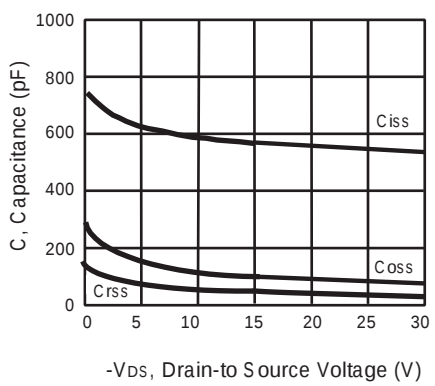
Figure 3. Capacitance
