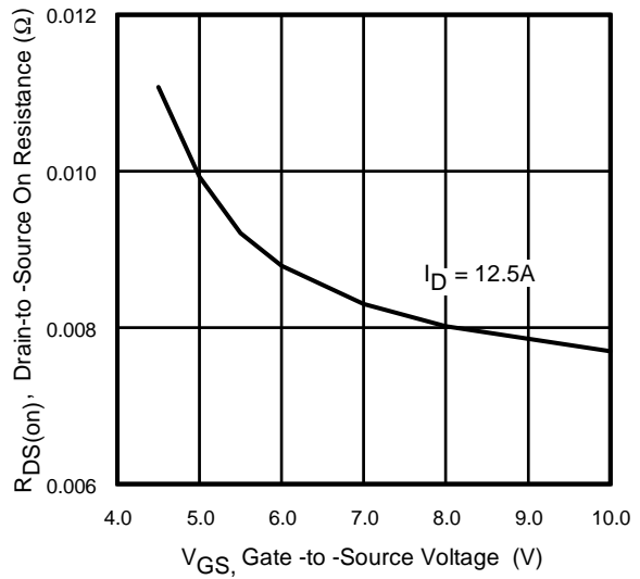
Fig 13. Typical On-Resistance Vs. Gate Voltage
