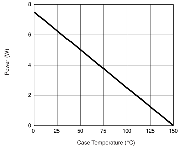
Power Derating
