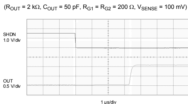
Figure 7. Startup Delay
