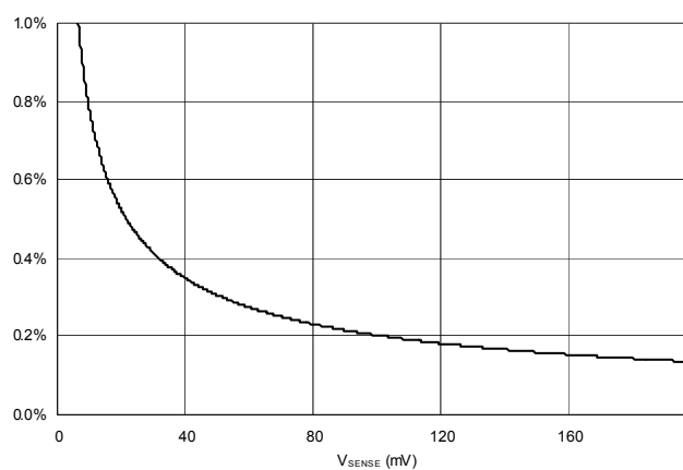
Figure 10. Output Error vs. Sense Voltage
