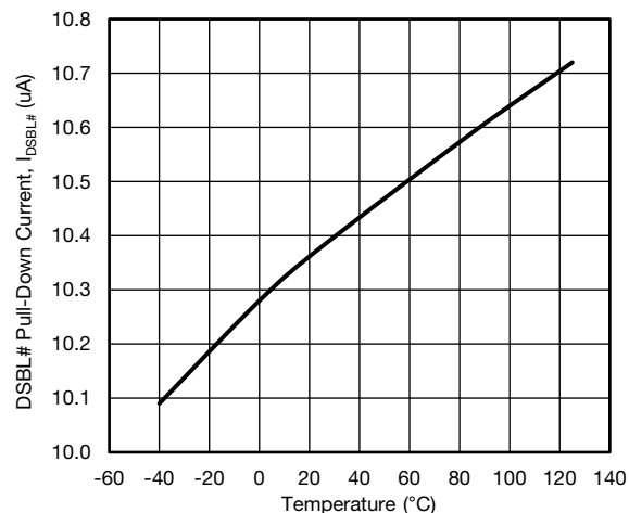
Fig. 14 - DSBL# Pull-Down Current vs. Temperature
