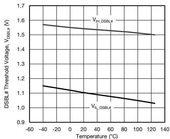
Fig. 12 - DSBL# Threshold vs. Temperature
