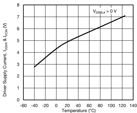
Fig. 16 - Driver Shutdown Current vs. Temperature
