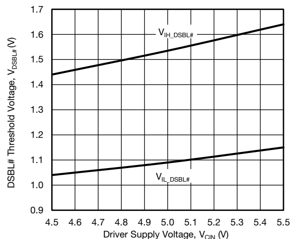
Fig. 13 - DSBL# vs. Driver Input Voltage
