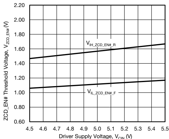
Fig. 15 - ZCD_EN# Threshold vs. Driver Supply Voltage
