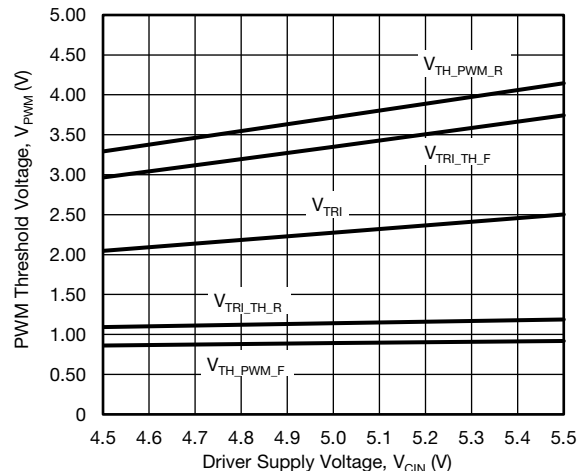
Fig. 11 - PWM Threshold vs. Driver Supply Voltage (SiC629)
