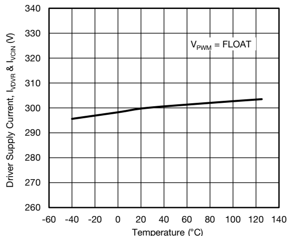
Fig. 17 - Driver Supply Current vs. Temperature
